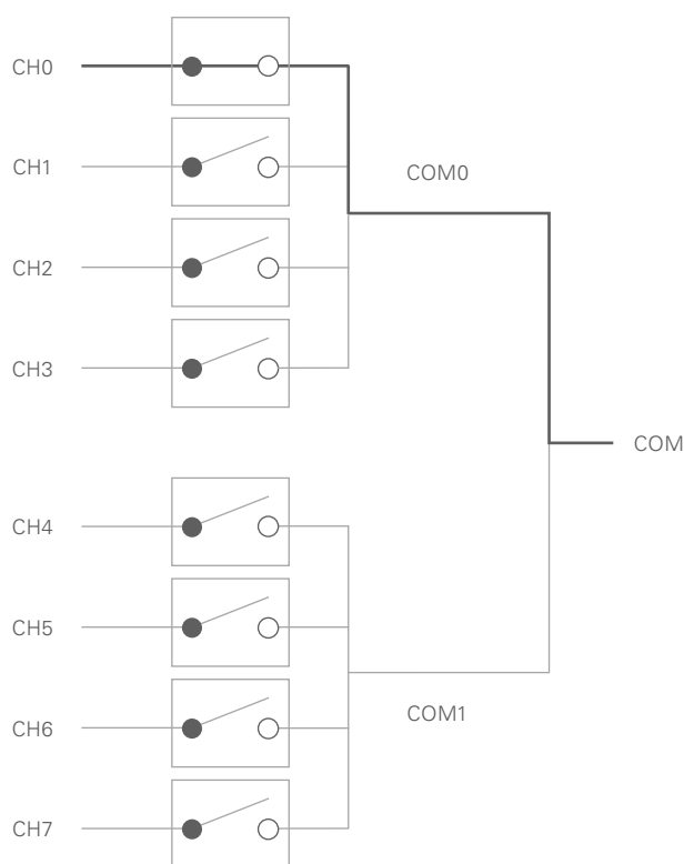
FIG 19 An 8 x 1 multiplexer is created by tying together the COMs of two 4 x 1 multiplexers.
