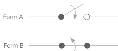
FIG 7 | SPST relays come in two forms: normally open (Form A) and normally closed (Form B).
