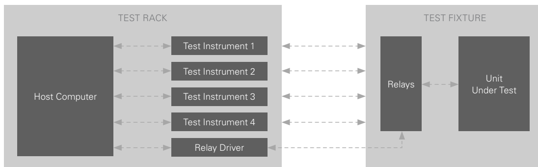
FIG 3 | Test systems with switches in the test fixture require a relay driver.
