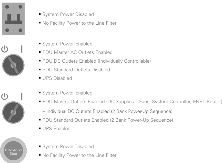
FIG 9 A test system requires multiple power states including off, enabled, on, and EPO to ensure efficient operation.
