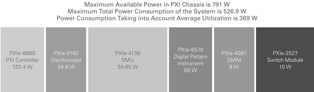
FIG 6 The total power consumption of a PXI Chassis is the sum of all modules in the chassis. You can see above a full chassis of instrumentation that will, in the worst-case scenario, consume 526.9 W.
