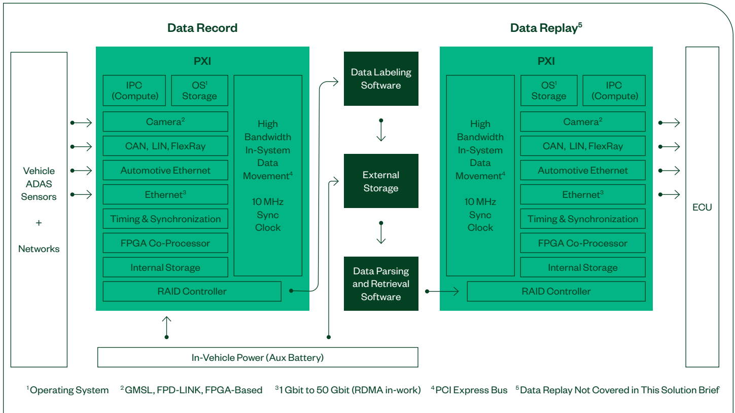
FIGURE 01 Block Diagram for Data Record Applications
