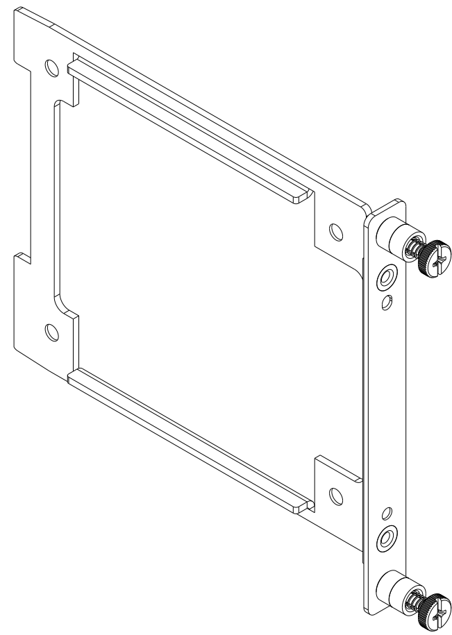
ISOMETRIC VIEW SHUTTLE, REMOVABLE HDD
