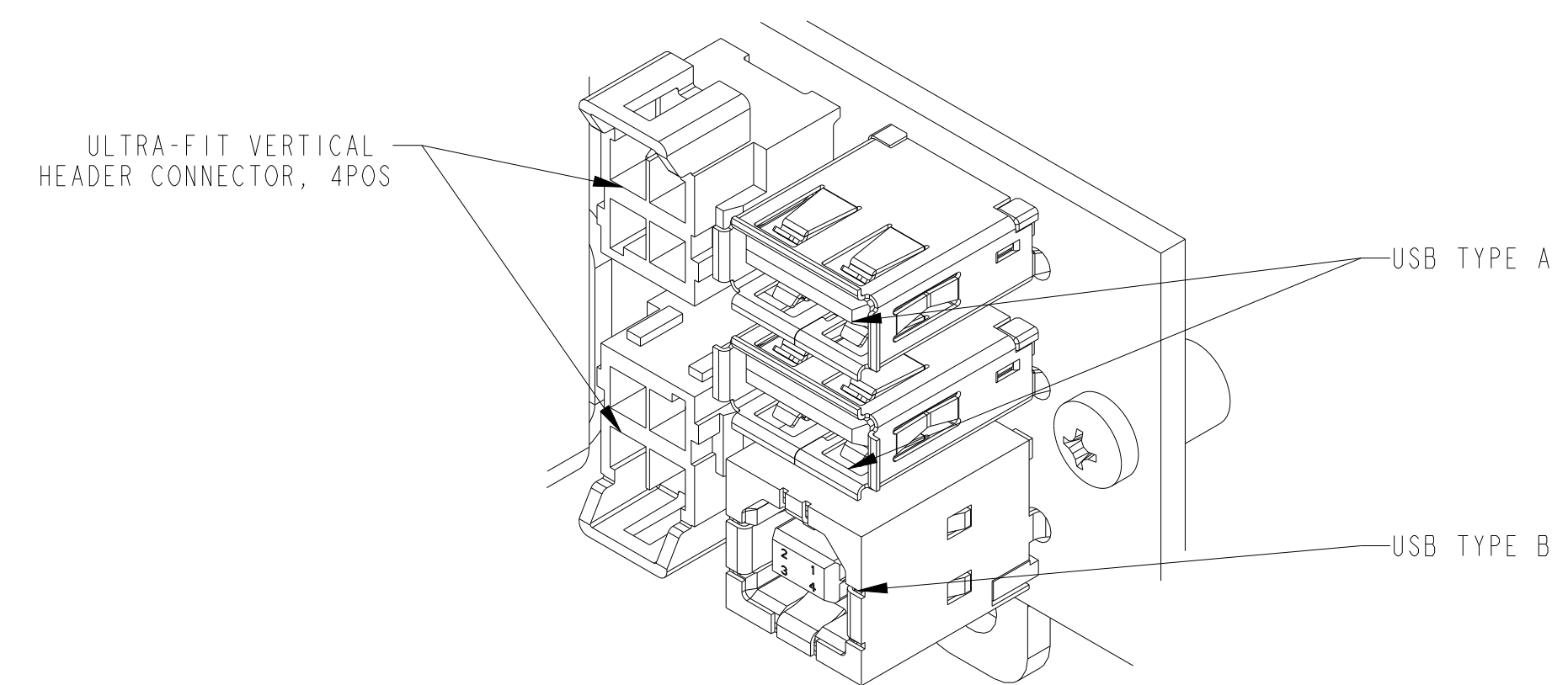
DETAIL A SCALE 5/2
