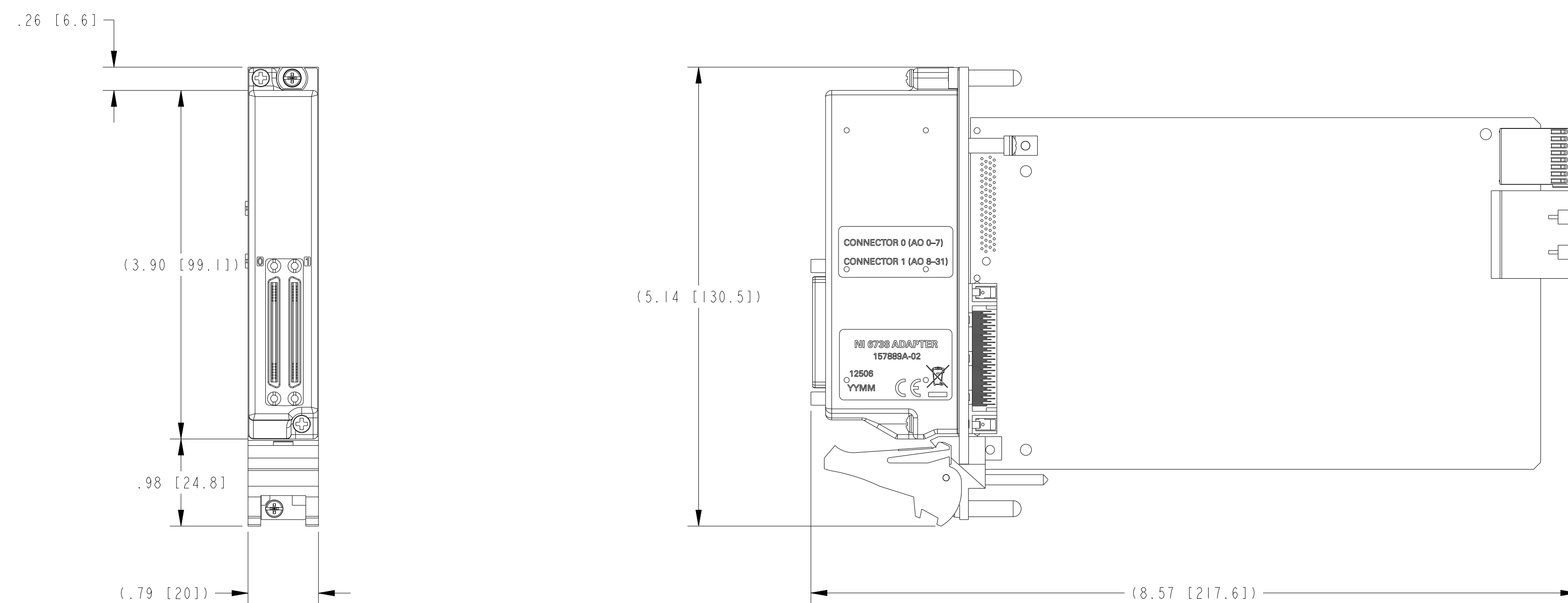
NI 6738 ADAPTER ASSEMBLED TO PXIe-6738
